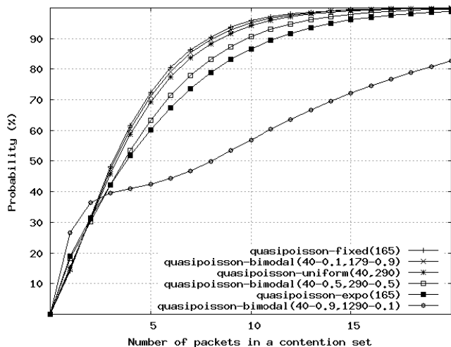
Figure 5: CDF of the number of packets in a contention graph for Poisson arrival with multiple distributions of packet length (mean = 165). The distribution with lower variance is listed first.
