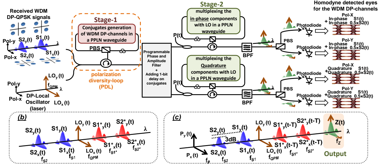
Fig. 1: (a) Concept of homodyne detection of WDM DP-signals utilizing PPLN waveguides inside polarization-diversity loops to coherently multiplex the signals, conjugates, and LO. The generated multi-level eye diagrams at the photodiode outputs correspond to multiplexing the in-phase and quadrature data on both polarization states, respectively, of the two channels. (b) Conjugates generation in Stage-1 using a dual-polarization LO in a PDL. (c) Multiplexing of the DP-signals, conjugates and LO using a DP-pump ( P(t) ), and PPLN waveguides inside two PDLs (for the in-phase and quadrature paths) in Stage-2.
