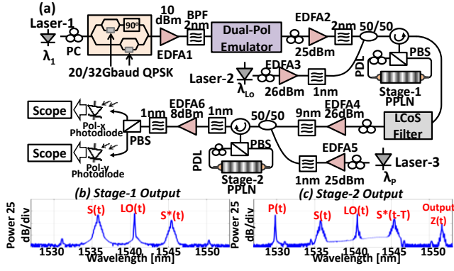
Fig. 2: (a) Experimental setup for a homodyne receiver for a DP-QPSK signal using PPLNs inside a PDL. (b) Experimental spectrum after the first stage (Stage-1). (c) Experimental multiplexing spectrum after Stage-2.
