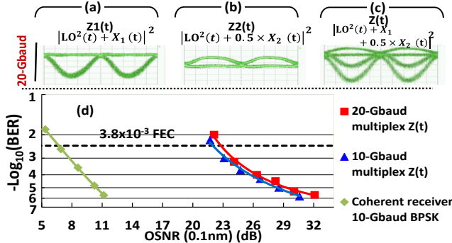
Fig. 5: (a) Experimental homodyne detection eyes for the first BPSK signal. (b) Detected eyes for the second BPSK signal. (c) The multiplexed four-level eyes composed of two BPSK signals at 20 Gbaud. (d) BER performance of the four-level multiplexed output.
