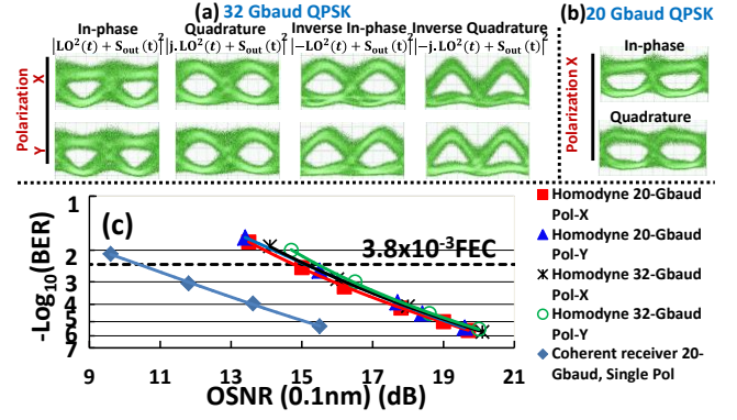
Fig. 3: Experimentally recorded eyes the from homodyne detection of a DP-QPSK signal showing the I/Q components under different conditions at (a) 32 Gbaud, and (b) 20 Gbaud. (c) BER performance of the homodyne detection system and the BER measured using a coherent receiver.
