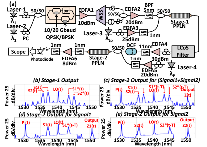
Fig. 4: (a) Experimental setup of homodyne detection for two SP-PSK signals using nonlinearity. (b) Spectrum after conjugate generation in Stage-1. (c) Spectrum of the multiplexing of both signals with LO after Stage-2. (d,e) Multiplexing spectra when only one signal/conjugate pair is transmitted at the LCoS filter while the other pair is blocked.
